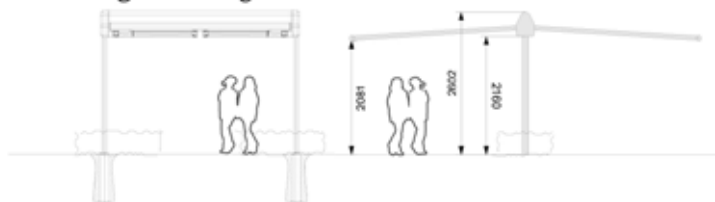
detaillering zonwering
